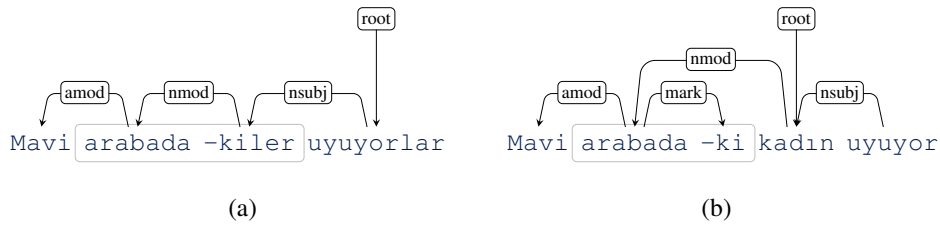
Figure 3: Dependency analyses of sentences in (2), demonstrating a nominal (a) and adjectival (b) derived with the suffix -ki .
