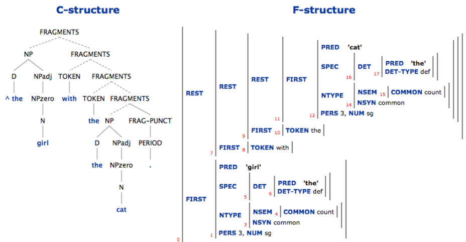
Figure 1: The FRAGMENT LFG analysis of ‘The girl with the the cat.’
