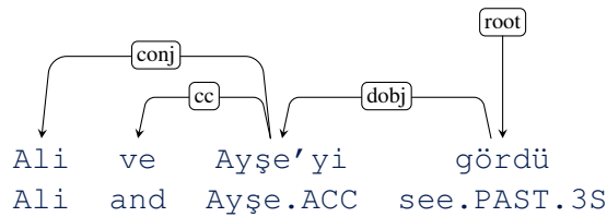
Figure 7: The analysis of sentence ‘She/he saw Ali and Ayşe’. Note that annotating Ali as the head would make it difficult to search for accusative subjects, or mislead a parser to assign a subject relation rather than object, since the relevant feature is not immediately available on the head as it is in majority of the other cases. The problem becomes more severe when there are more than two conjuncts, and in case of covert coordination where no explicit conjunction or punctuation exists.
