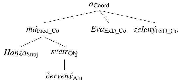
Figure 1: The input dependency structure of (7)
