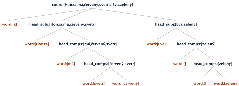
Figure 4: The structure for (7) after it is checked by the grammar
