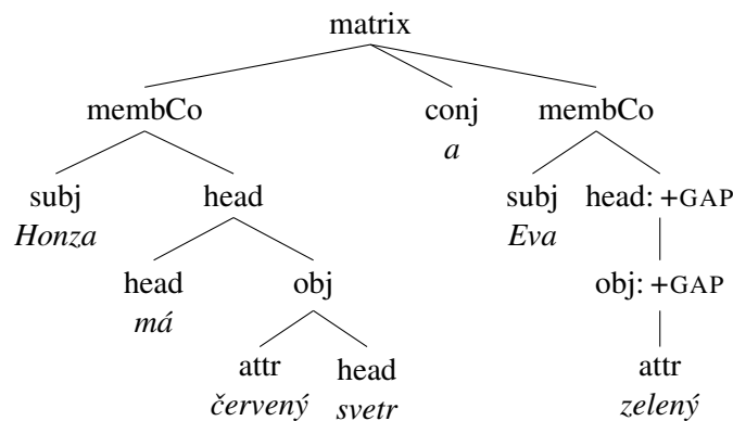
Figure 2: Example (7) after conversion to constituency structure, with restored mother nodes in the clause Eva _ zelený _ ‘Eva a green one’
