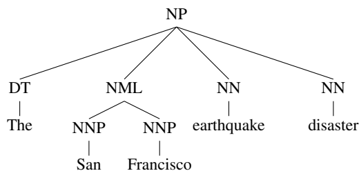
Figure 1: Internal noun phrase structure
