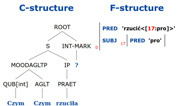
Figure 2: Czym rzuciła? – structures for interpretation (2), Ron Kaplan's tokeniser.
