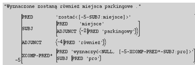
Figure 8: The recomposed f-structure of the FRAGMENT f-structure of Figure 6
