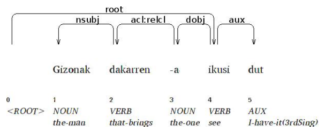
Figure 3: Alternative analysis of the sentence in Figure 1
