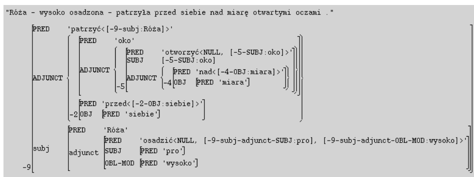
Figure 3: The recomposed f-structure of the FRAGMENT f-structure of Figure 2; dependency labels used as new attributes are written in lower case
