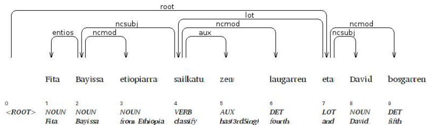
Figure 5: Analysis in the BDT where the conjunction is the head and and acts as a place holder for ellipsis ( Fita Bayissa from Ethiopia has classified fourth and David fifth ).
