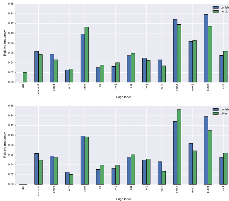
Figure 3: Dependency labels distribution comparison for Danish vs. Nordic Swedish and Norwegian (above), and for Danish vs. all languages (below).
