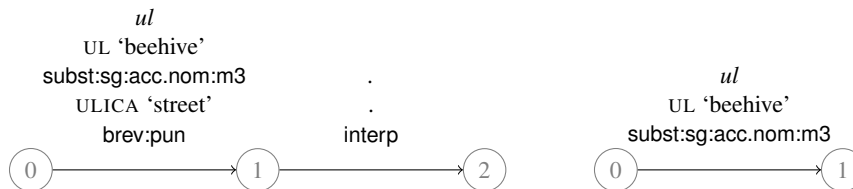
Figure 5: Morfeusz analyses of ul . (left) and ul (right).
