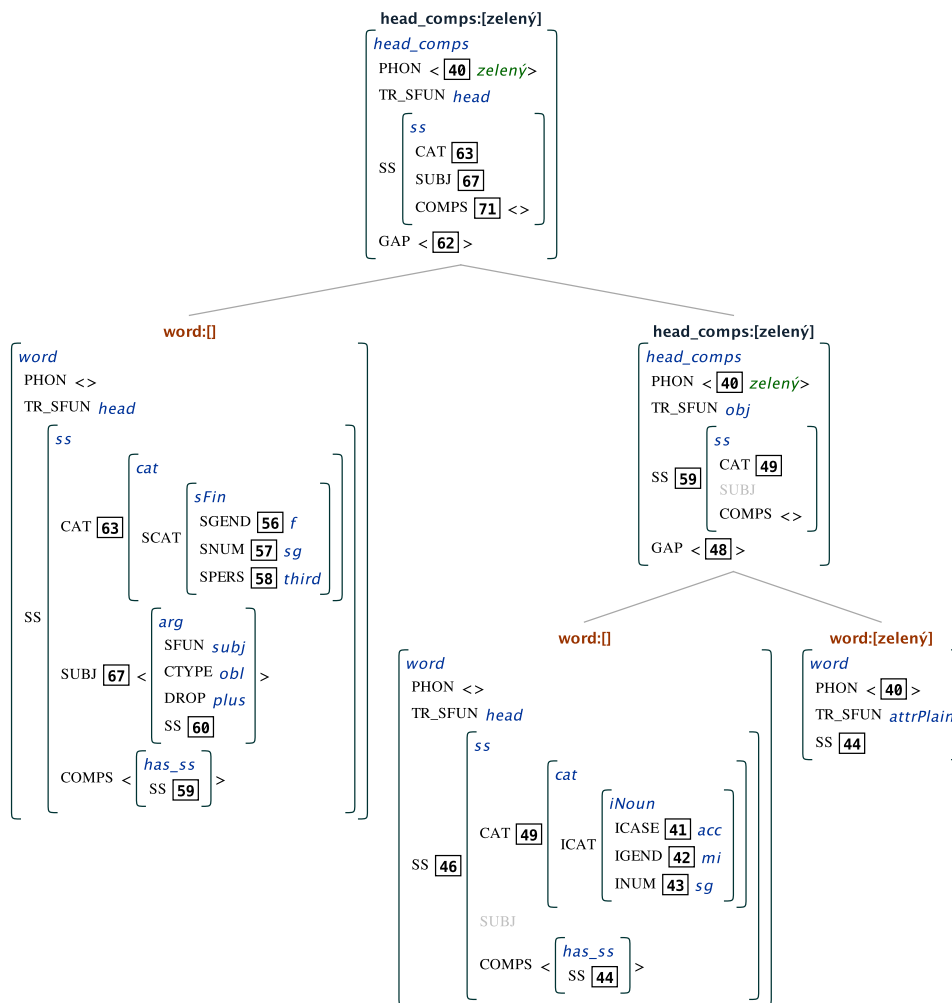
Figure 5: A part of Fig. 4 showing two instances of ellipsis
