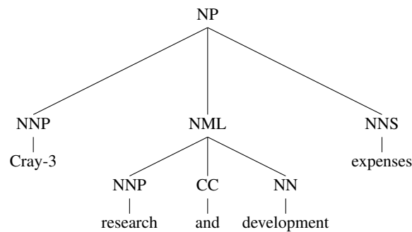
Figure 3: Coordination structure: Left-branching
