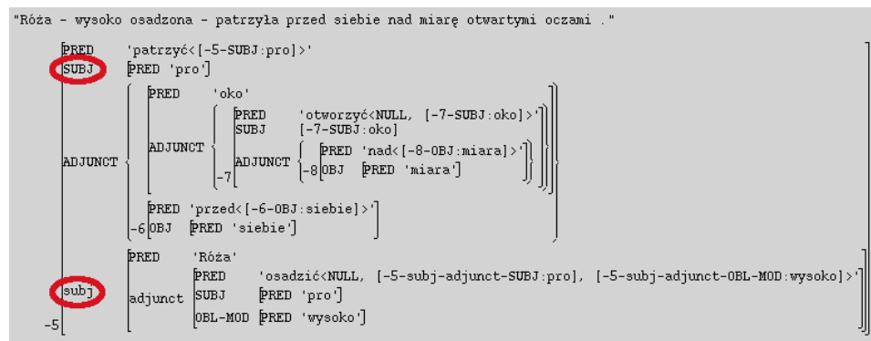
Figure 5: The incoherent f-structure glued from sub-f-structures in Figure 2
