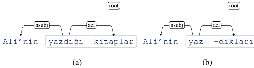
Figure 6: (a) A normal relative clause headed by a noun ‘the books Ali has written’. (b) A headless relative clause ‘the ones Ali has written’.
