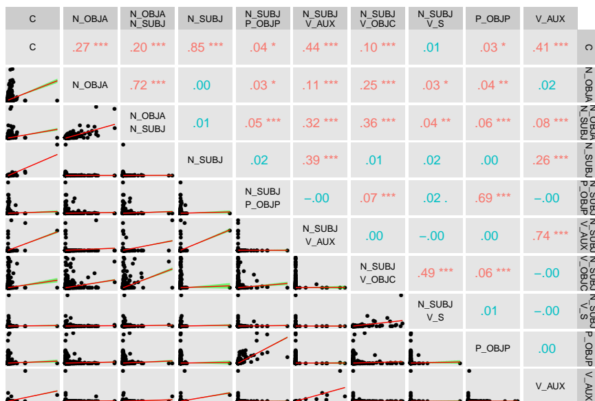
Figure 2: Correlations between the 10 most frequent verb valencies. Red magnitudes indicate statistically significant correlations. Stars indicate the p-values.
