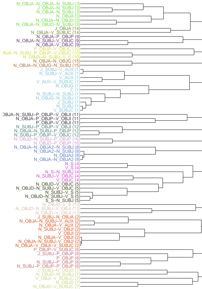
Figure 3: Clustering of the 70 most frequent valency patterns based on correlation scores. Numbers in brackets indicate cluster in order of cluster size. Clusters were extracted with a dynamic tree cutting algorithm.
